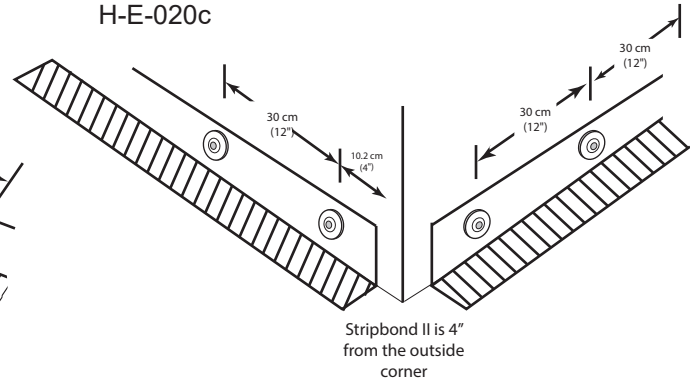
Hi-Tuff TPO Stripbond II Outside Corner H-E-020c
