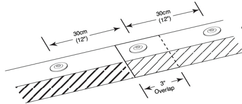
Hi-Tuff TPO Stripbond II Ends H-E-020a
